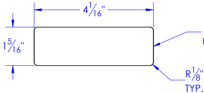
FP-HFL-235 END CAP END CAP, EXTENSION, HYDRA FLAKER 12ga HRS.
